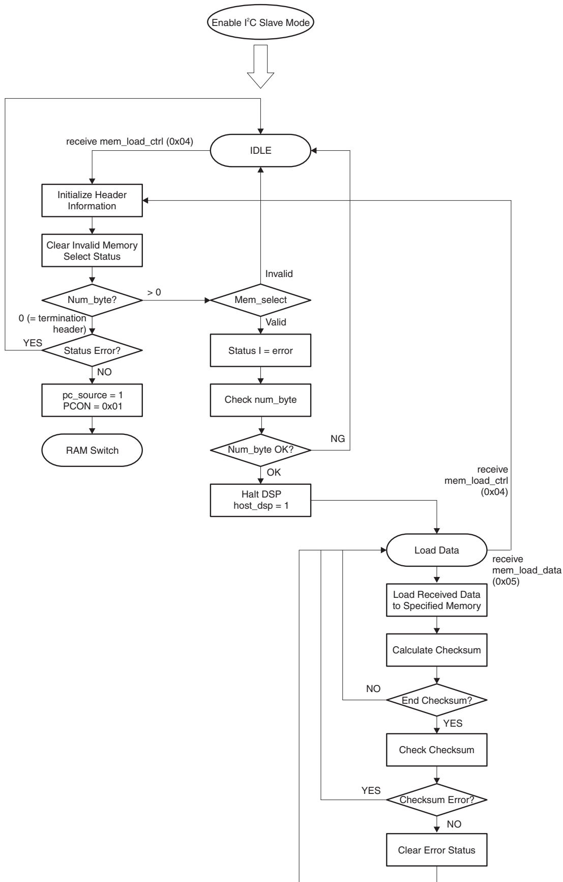
Figure 39. I 2 C Slave Download Flow
