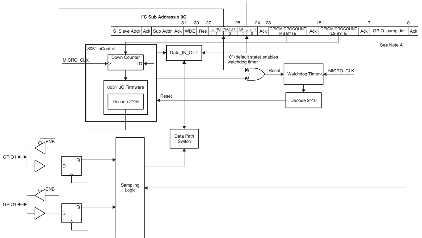
Figure 18. GPIO Ports
